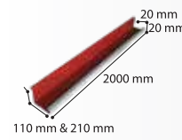
Eco Baca Dibi Profili Eco Profile of Chimney Bottom
