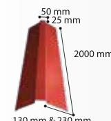
Eco Tepe Mahya Profili Eco Square Ridge Cape
