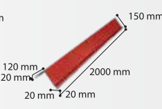
Eco Yan Saçak Mahya Profili Eco Barge Board Flashing
