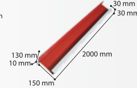
Eco Yan Saçak Mahya Vadi Dere Profili Eco Side Eave Roof Ridge and Valley Creek Profile
