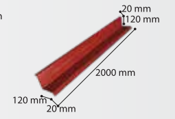
Eco Duvar Dibi Profili Eco Wall Side Flashing
